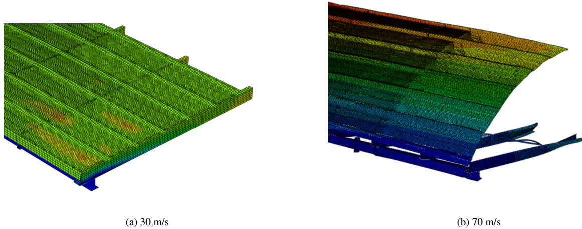
Figure 5: Roof corner deformed shapes at low and high wind speeds
