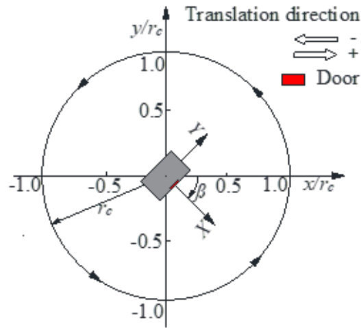
Figure 3: Experiment configuration
